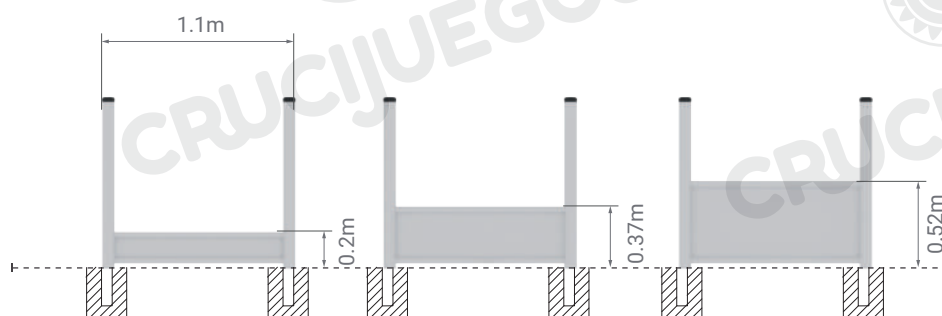
Vista frontal:
